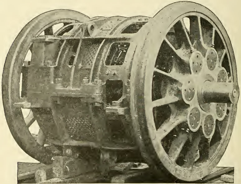
Fig. 254. Motor Mounted on Its Axle
